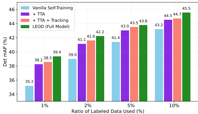
(a) Gen1 weakly-supervised object detection (WSOD) results
